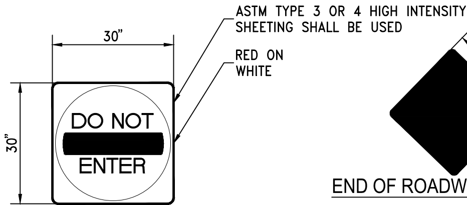
DO NOT ENTER SIGN TYPE R5-1
